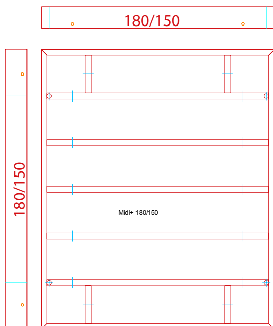
Midi + 180ht x 150
